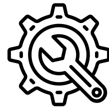
Software Troubleshooting
